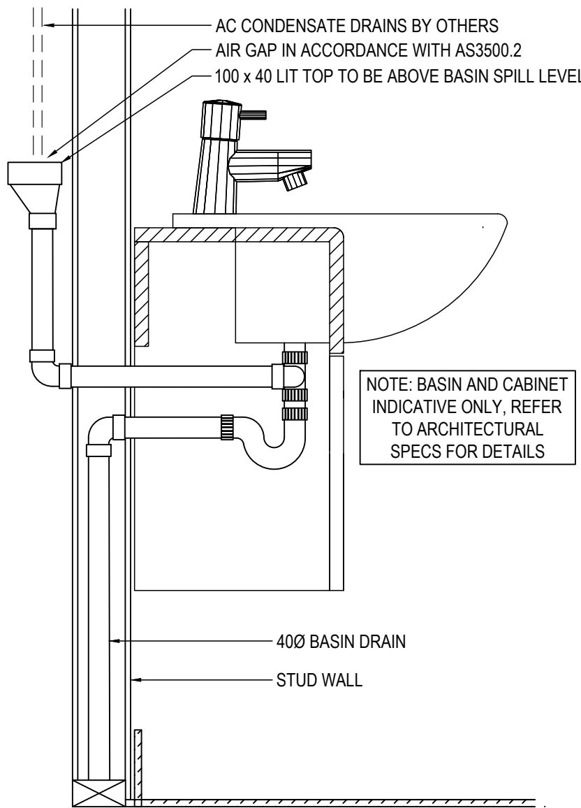
A/C WASTE WATER TUNDISH DETAIL (TD-1) NOT TO SCALE
